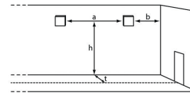
Wandmontage
